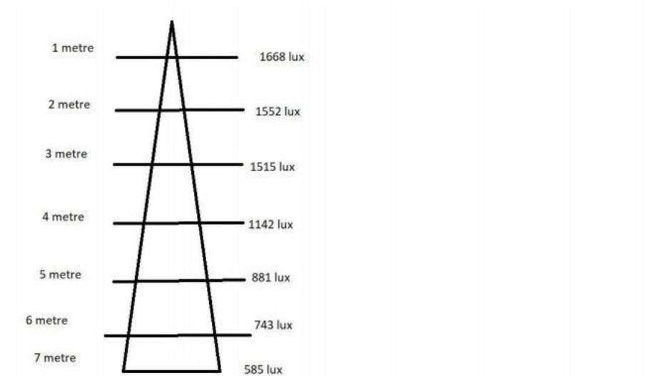
Figure 2. Cone diagram for mounting height up to 8 metres. Based on peak beam intensity @ 30 degrees.
