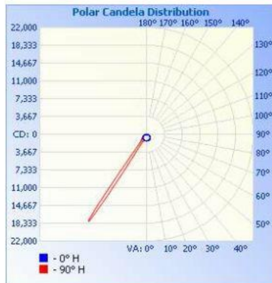
Figure 1. Polar Diagram
